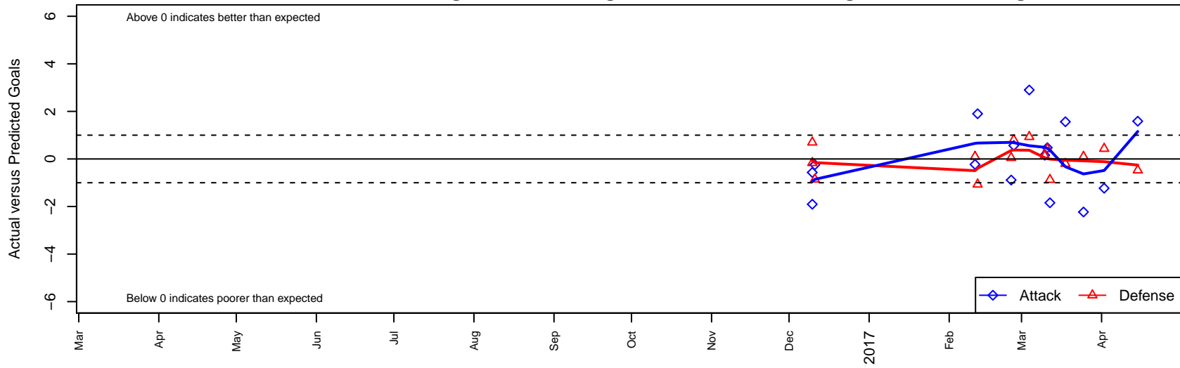
Sting SC Timbers G00 Dots are actual minus expected GF (blue circles) and GA (red triangles). Blue line is smoothed change in attack strength. Red is smoothed change in defense strength.
